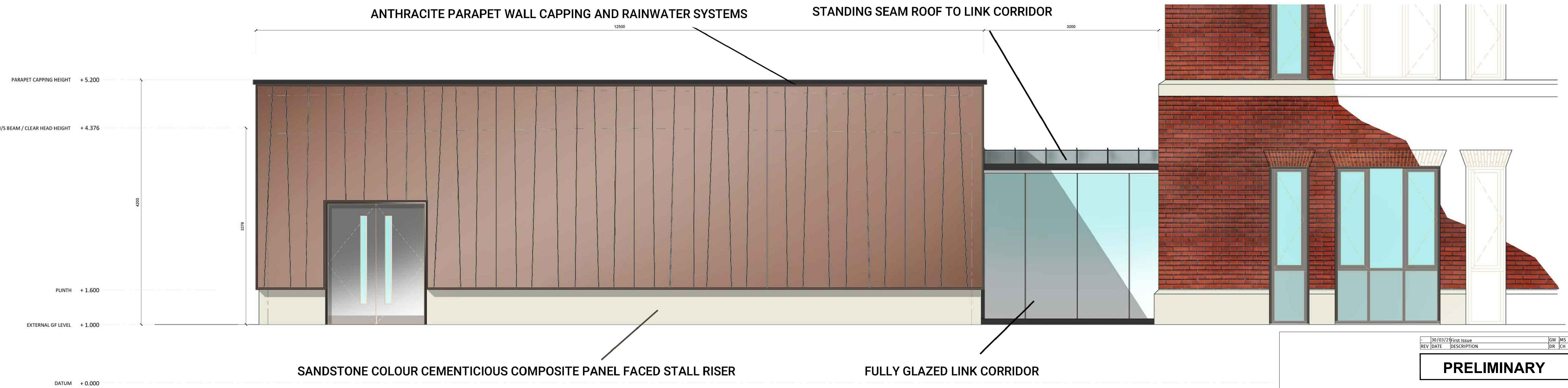
ENGINEERED CLADDING - RECESSED SEAM WEATHER SCREEN FACADE SYSTEM IMAGES
