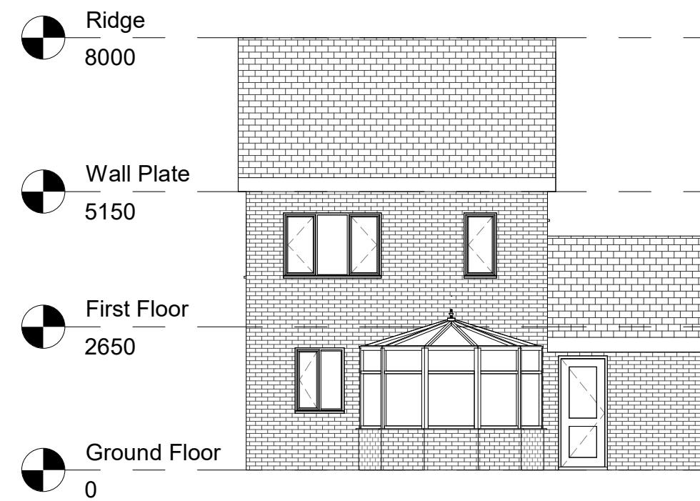
7 Existing Rear Elevation 1 : 100
