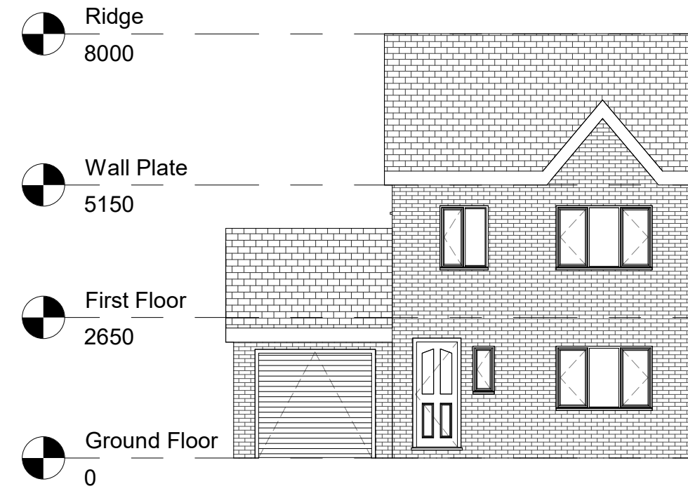
5 Existing Front Elevation 1 : 100
