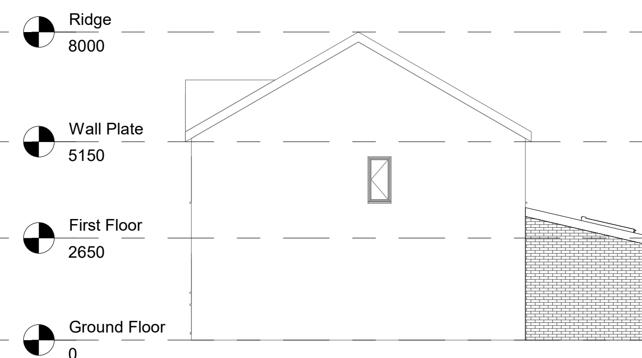
12 Proposed Right Side Elevation 1 : 100
