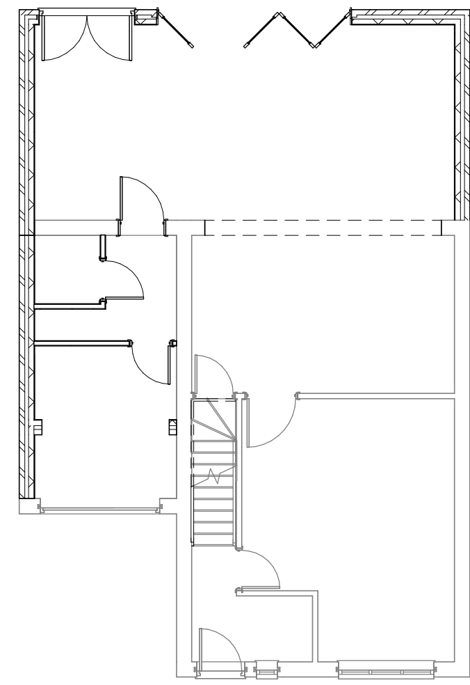
2 Proposed Ground Floor Plan 1 : 100
