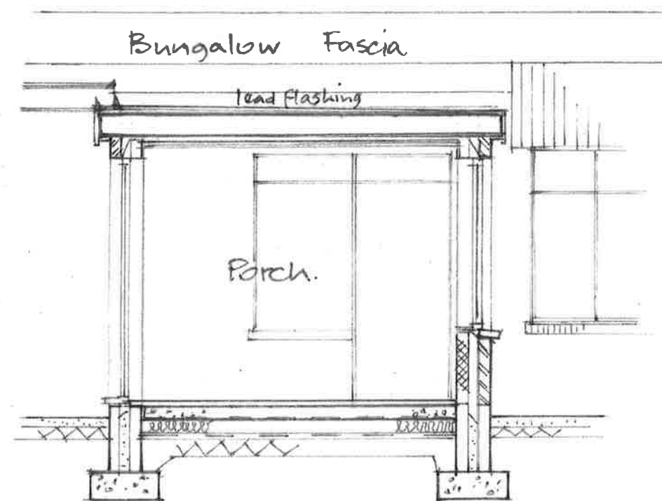
Section A-A (1:50)
