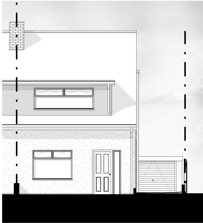
EXISTING FRONT
