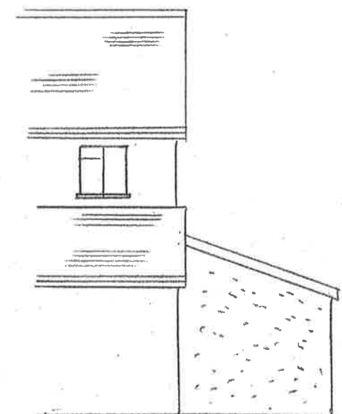
REAR ELEVATION EXISTING AND PROPOSED
