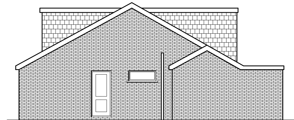
Proposed RH Side Elevation
