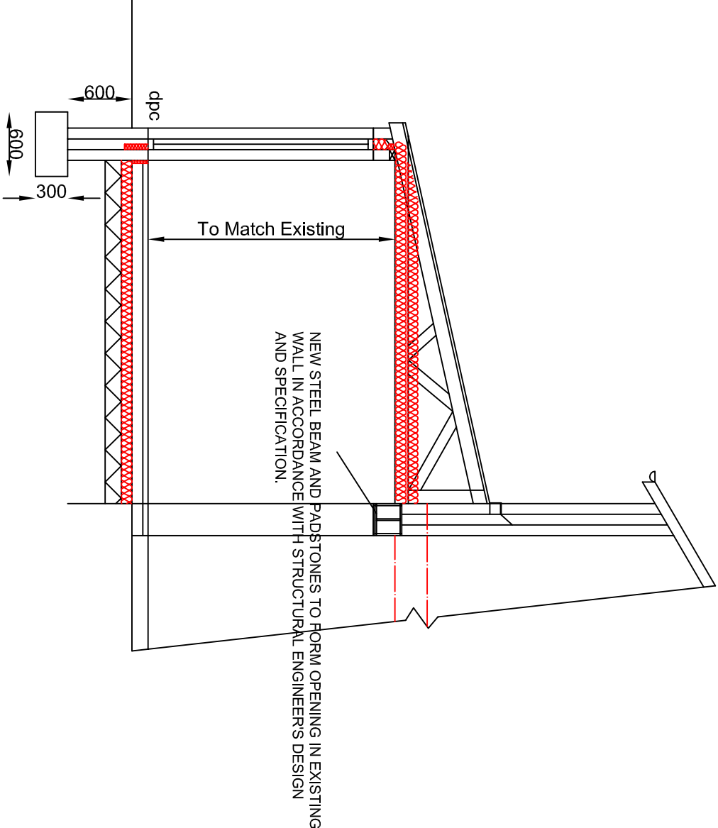
PROPOSED SECTION X-X
