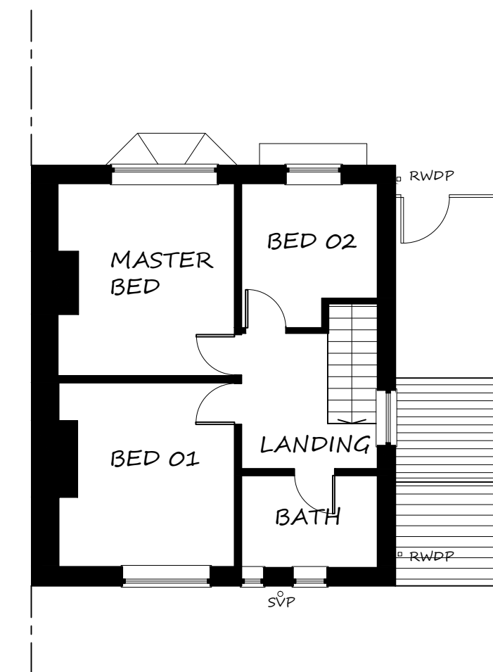
FIRST FLOOR PLAN AS EXISTING SCALE 1:100 @ A1
