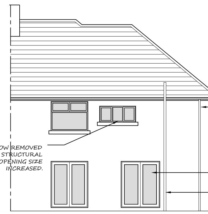
NORTH EAST ELEVATION AS PROPOSED SCALE 1:100 @ A1
