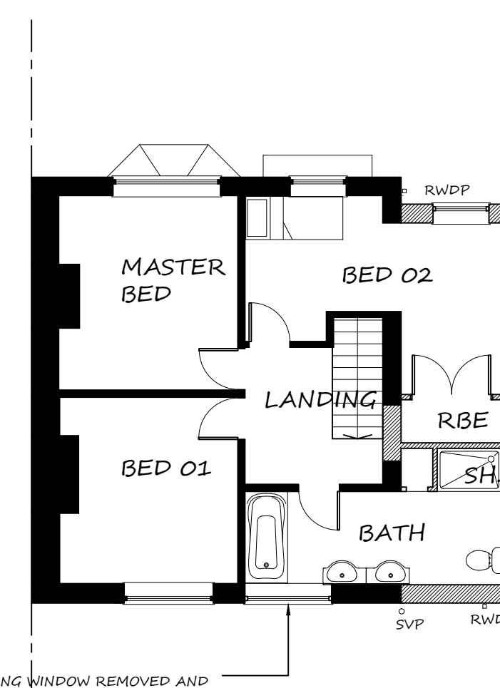
FIRST FLOOR PLAN AS PROPOSED SCALE 1:100 @ A1
