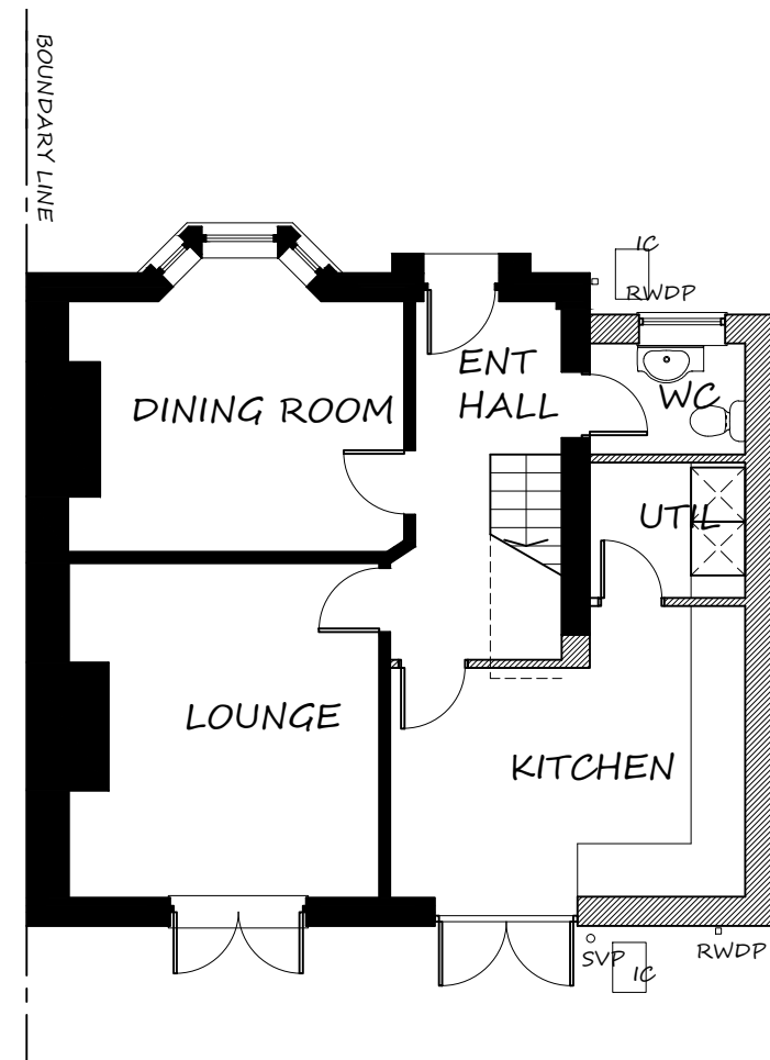
GROUND FLOOR PLAN AS PROPOSED SCALE 1:100 @ A1
