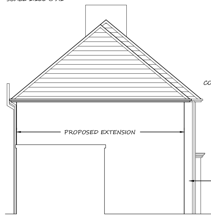
SOUTH WEST ELEVATION AS PROPOSED SCALE 1:100 @ A1
