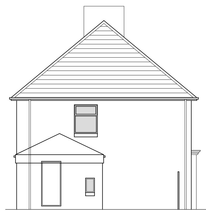
SOUTH WEST ELEVATION AS EXISTING SCALE 1:100 @ A1
