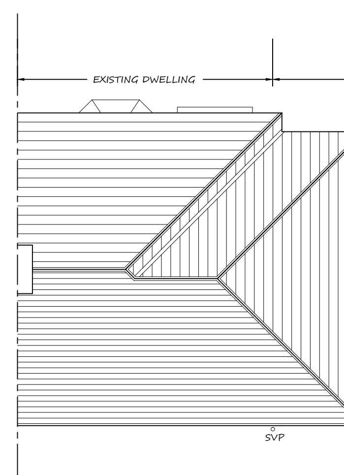
ROOF PLAN AS PROPOSED SCALE 1:100 @ A1
