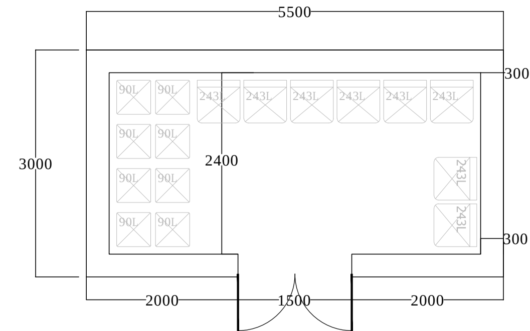
FLOOR PLAN
