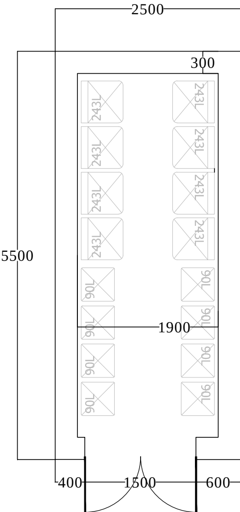
FLOOR PLAN
