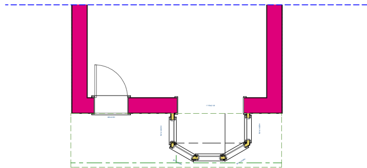
Partial floor plan as existing (1:100)
