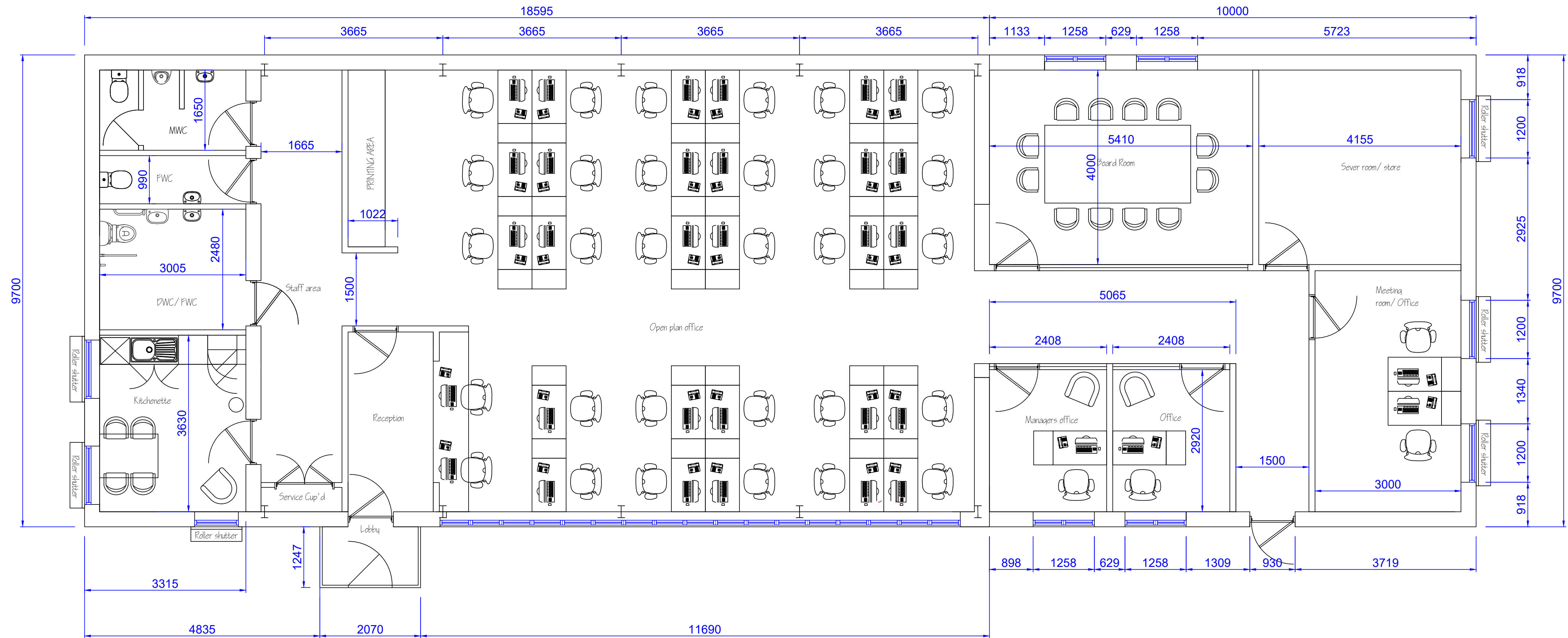
Ground Floor Plan 1:50
