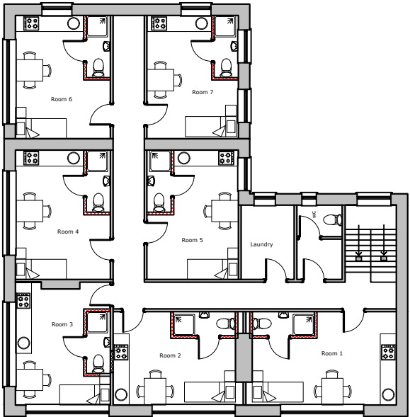
PROPOSED FIRST FLOOR Scale: 1:200
