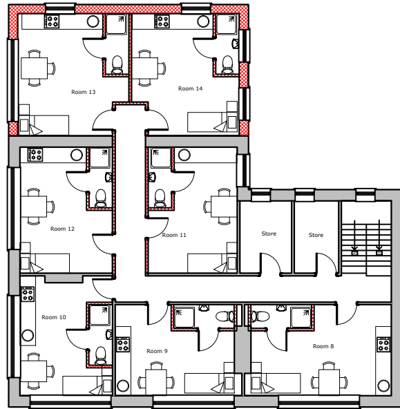
PROPOSED SECOND FLOOR Scale: 1:200
