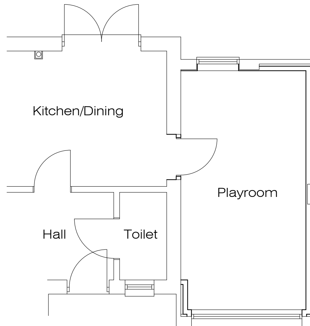
PROPOSED PART GROUND FLOOR PLAN
