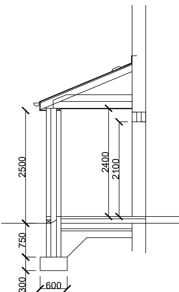
PROPOSED SECTION
