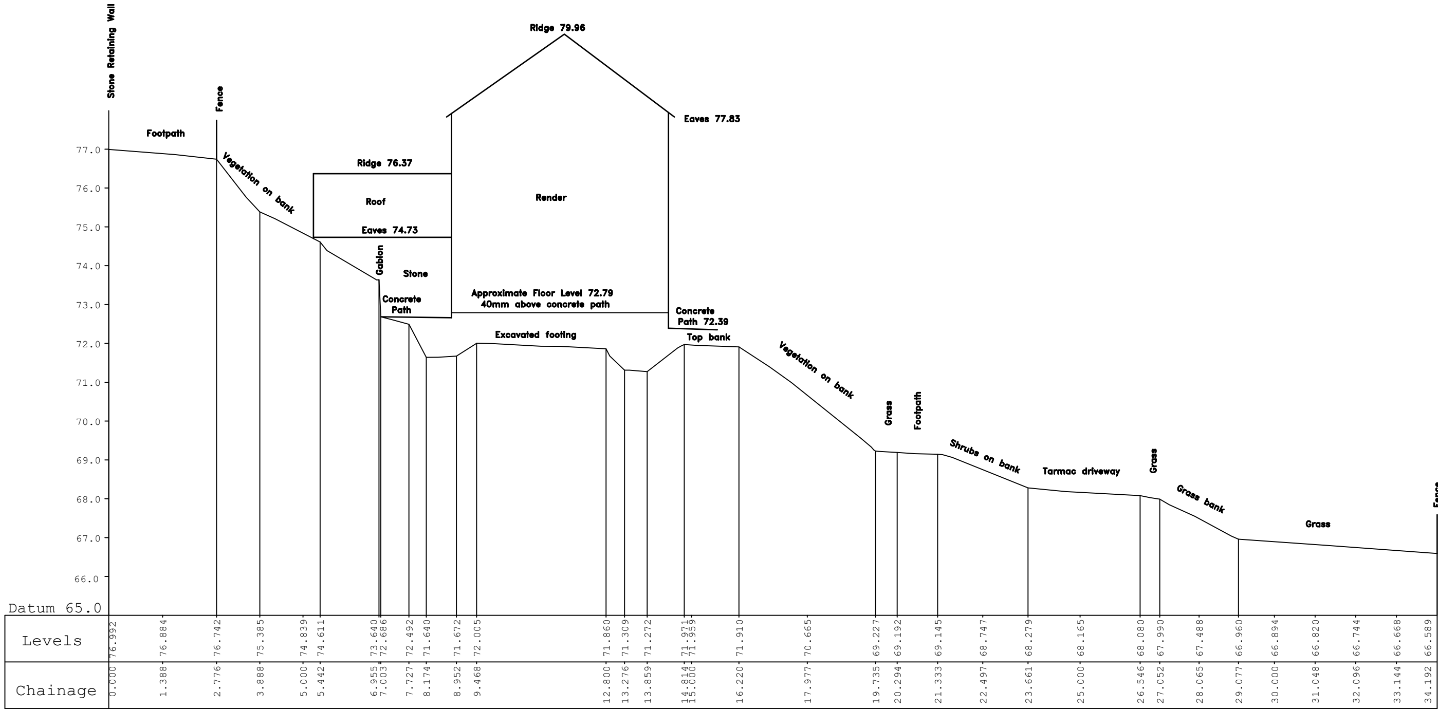
SECTION SCALE 1:100
