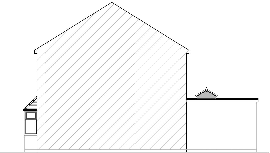
Proposed elevation on 'B' Scale - 1:100
