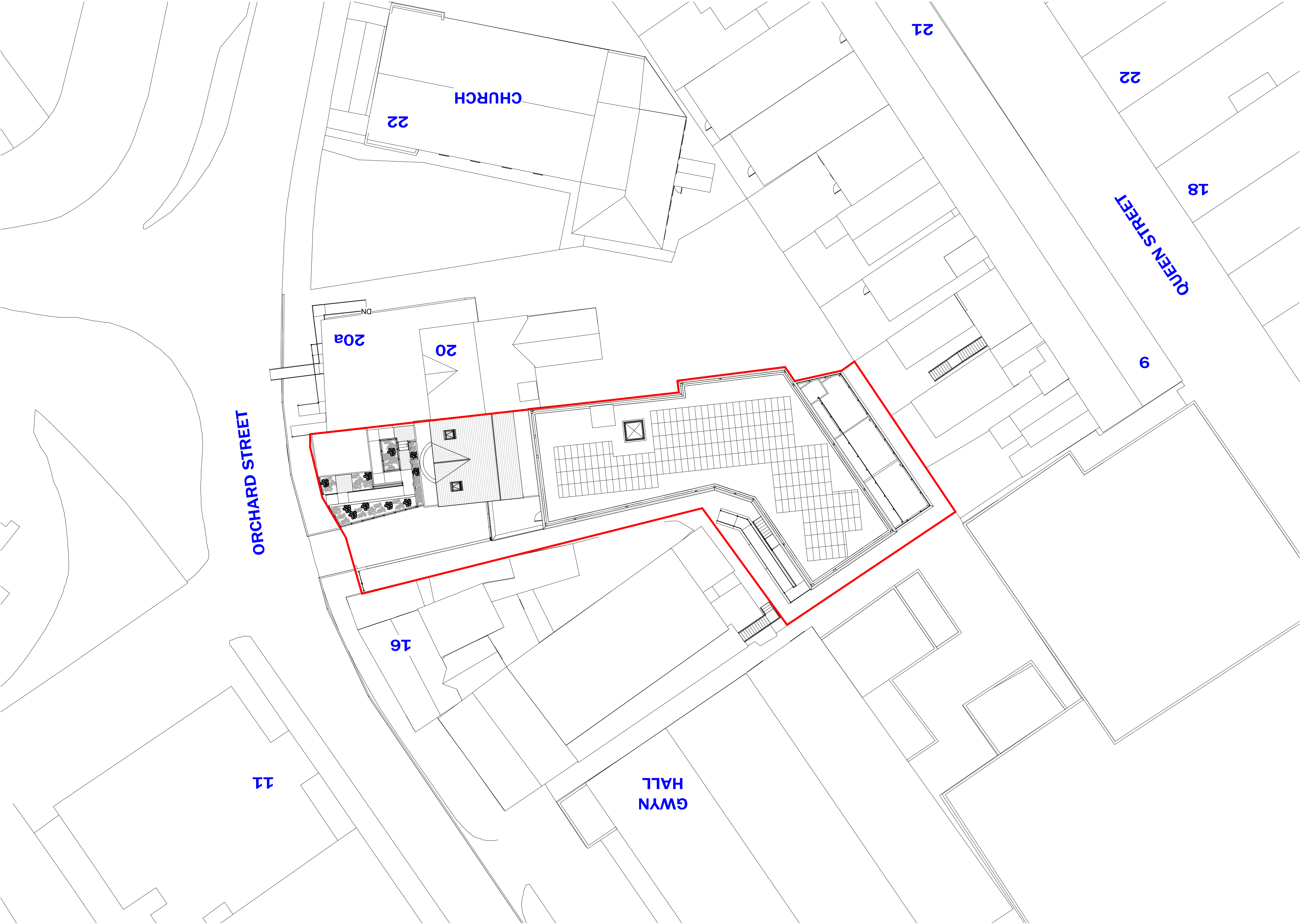
01 PROPOSED SITE LAYOUT 1 : 200
