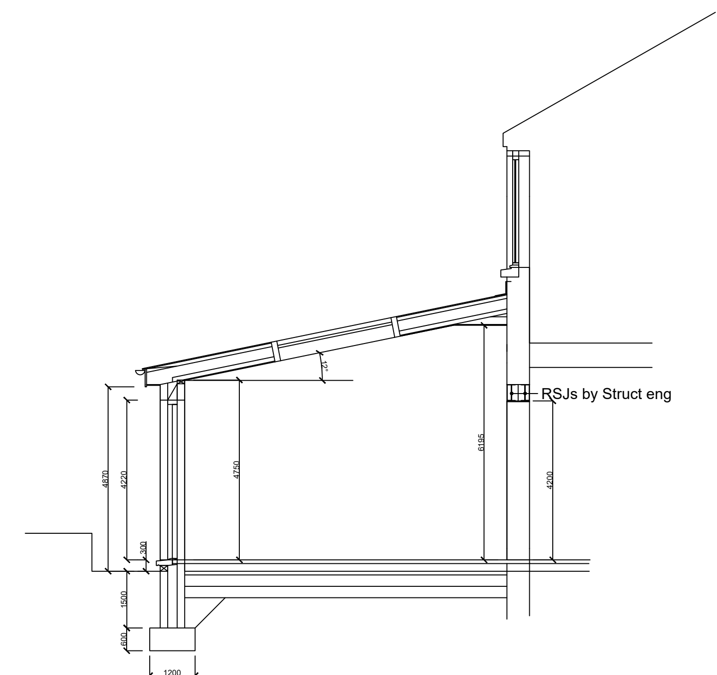
PROPOSED SECTION A-A 1:50 Scale
