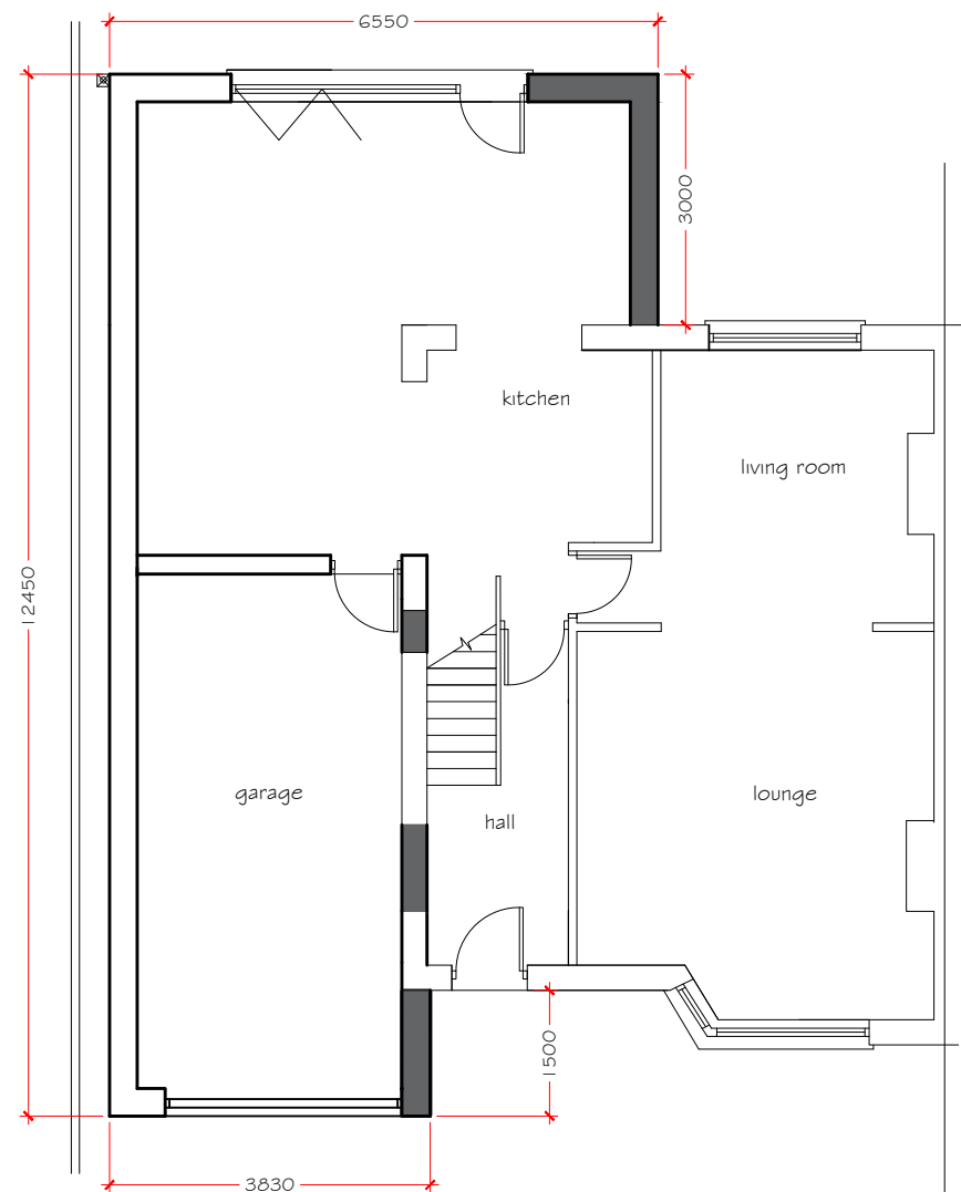
PROPOSED GROUND PLAN
