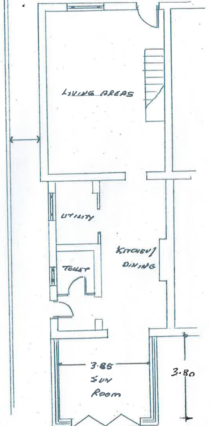
GROUND FLOOR PROPOSED
