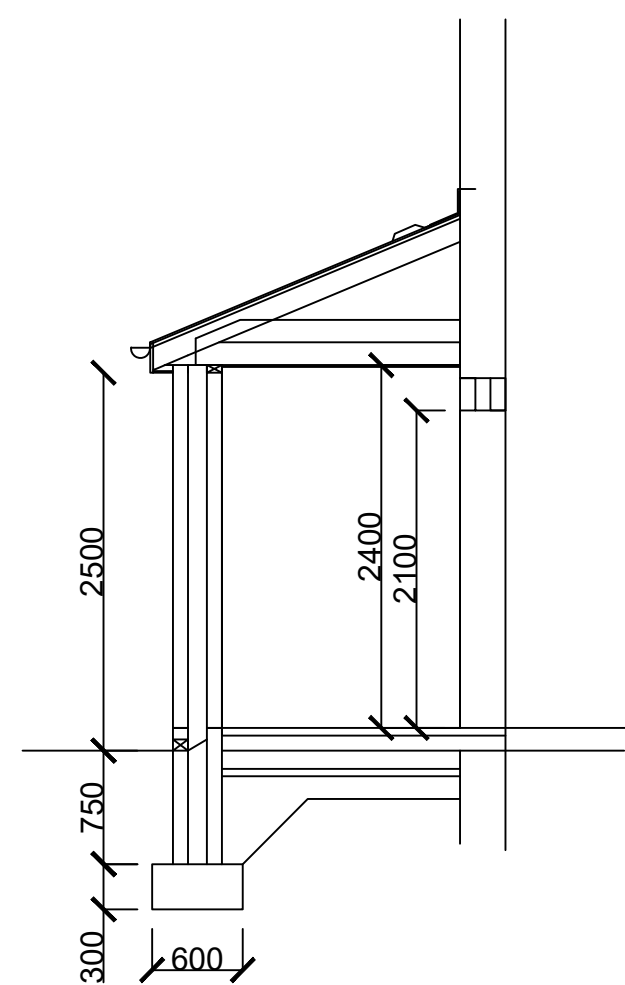
PROPOSED SECTION
