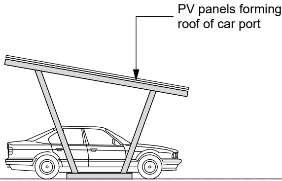
CROSS SECTION, 1:100
