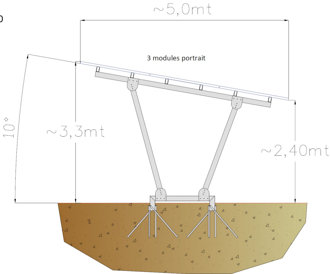
SIDE VIEW OF PROPOSED CAR PORT, N.T.S.
