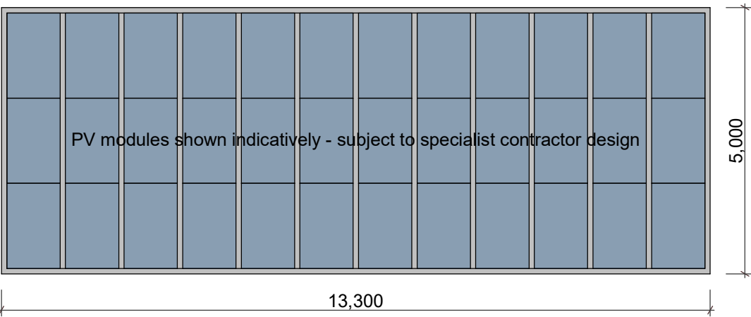
ROOF PLAN, 1:100
