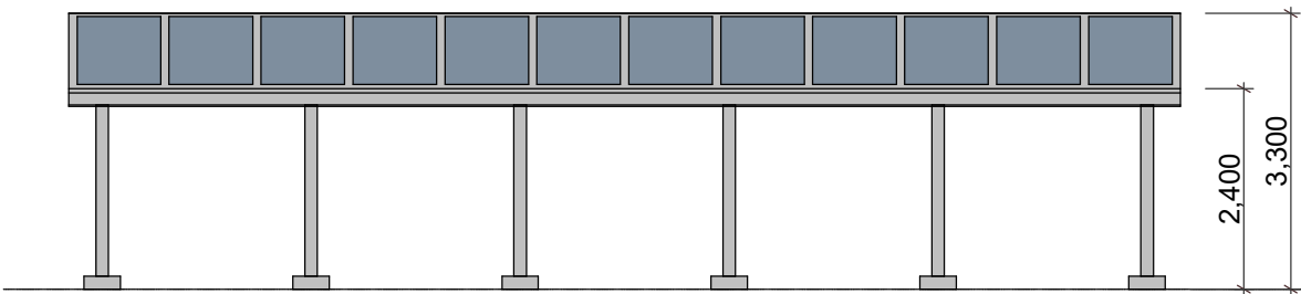
SOUTH ELEVATION, 1:100
