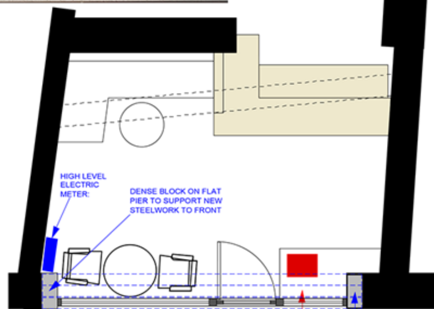
EXISTING PLAN 1:50
