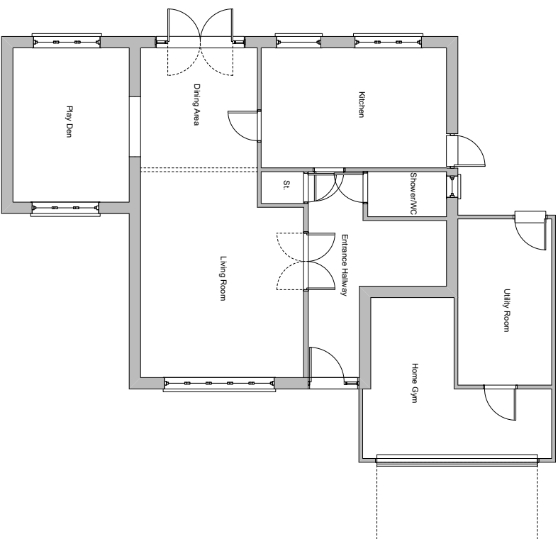
EX01.02 EXISTING GROUND FLOOR PLAN SCALE 1:50 @ A1, 1:100 @ A3
