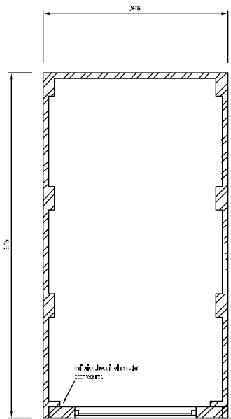
Typical Single Garage Floor Plan:
