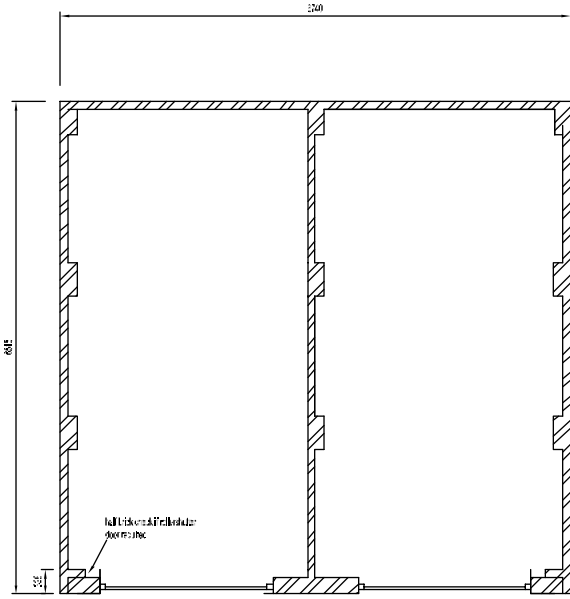
Typical Double Garage Floor Plan:
