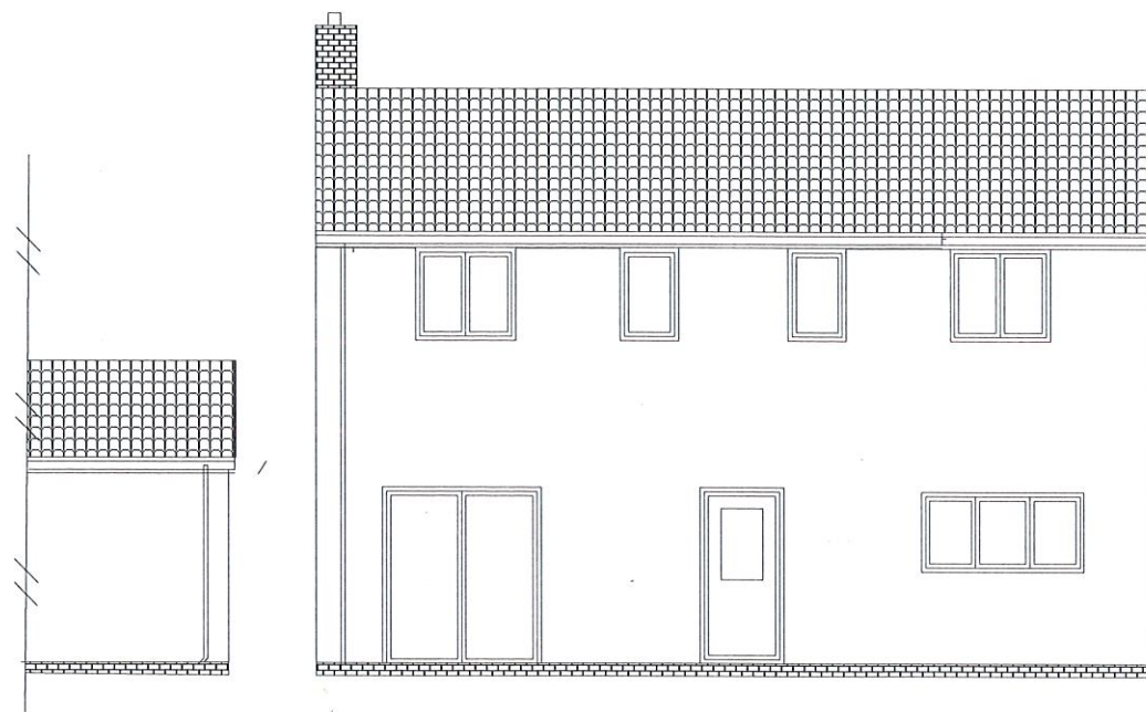
REAR ELEVATION
