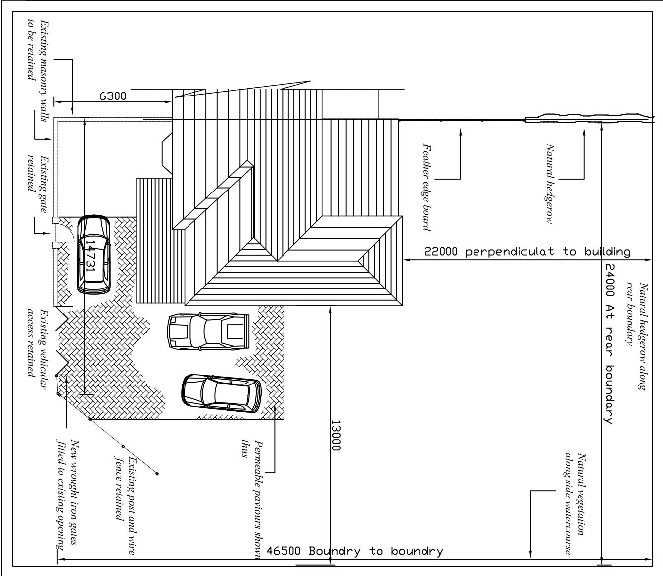
Block Plan @ 1 :: 200
