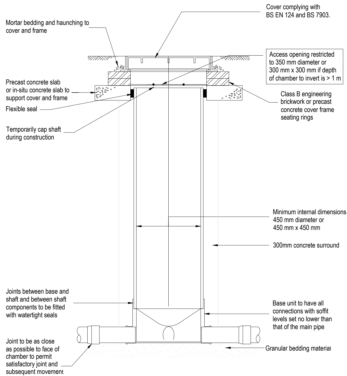
TYPE 3 (450-600 DIA.) INSPECTION CHAMBER
