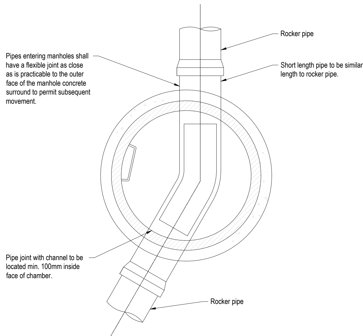
TYPICAL MANHOLE DETAIL - TYPE 2
