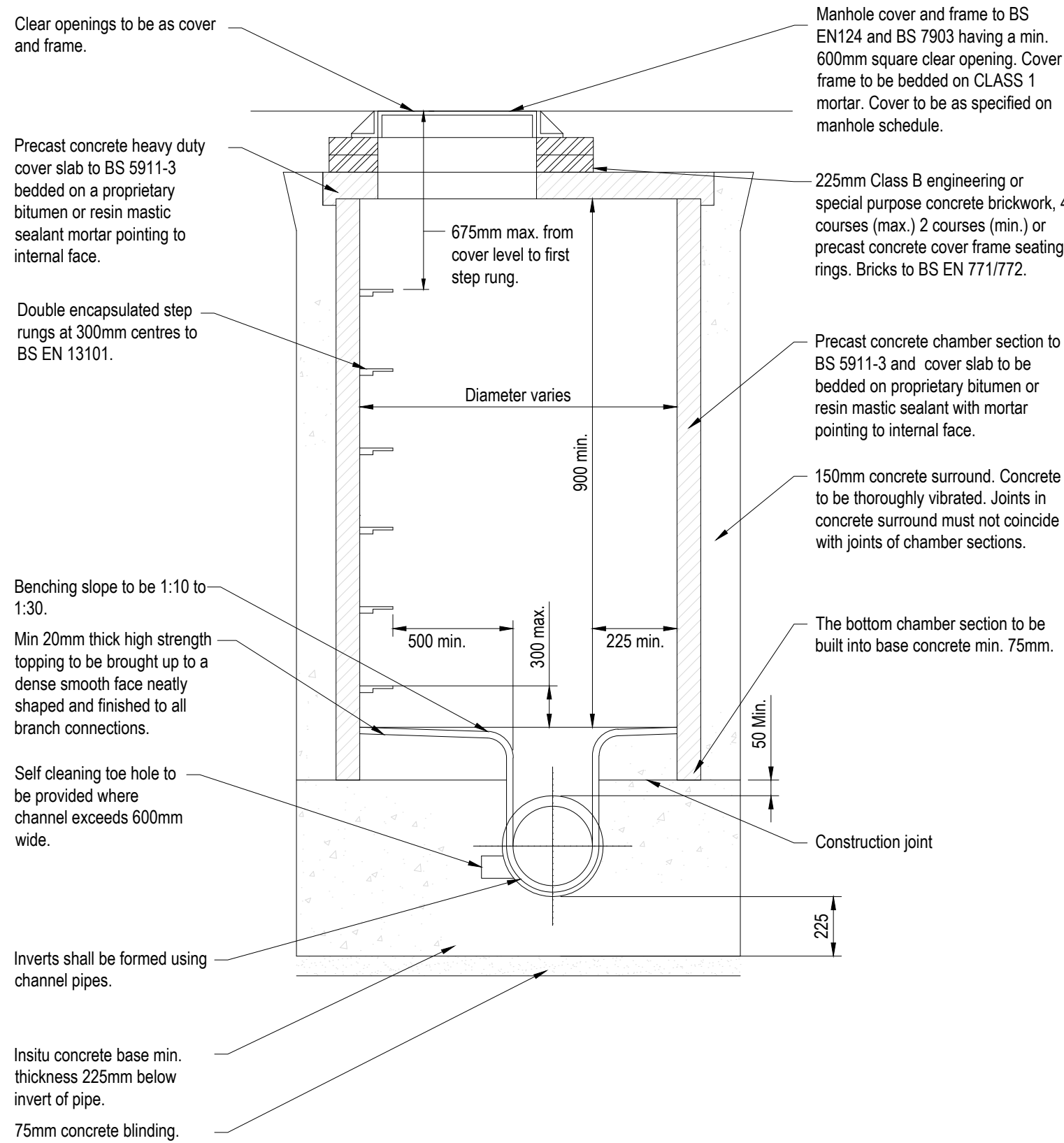
MH chamber sizes
