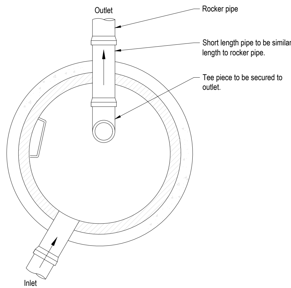
TYPICAL SILT TRAP DETAIL
