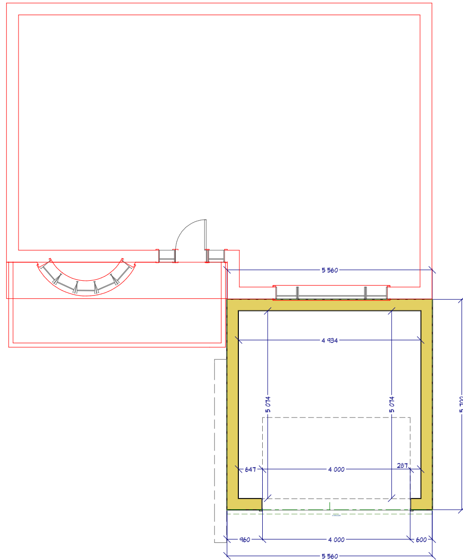
Existing garage
