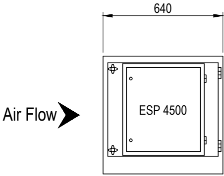
Front Elevation
