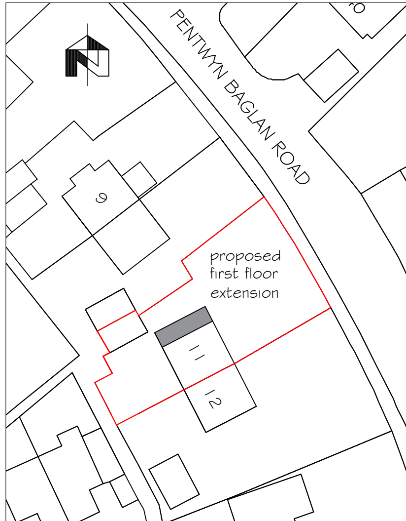
BLOCK PLAN 1:500
