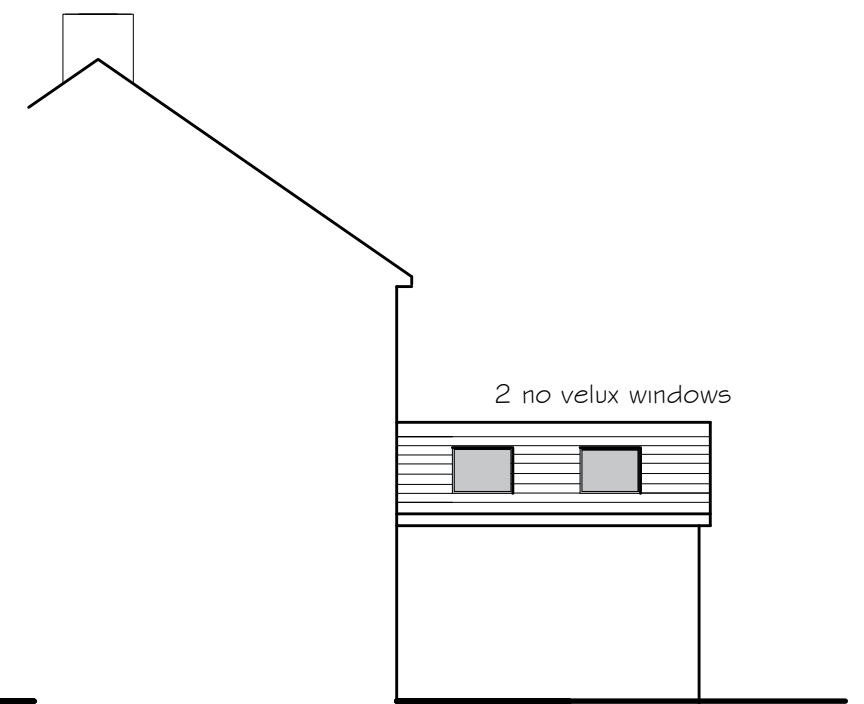
Proposed Elevation RHS
