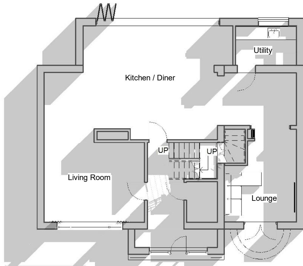
1 Proposed Ground Floor Plan 1 : 100
