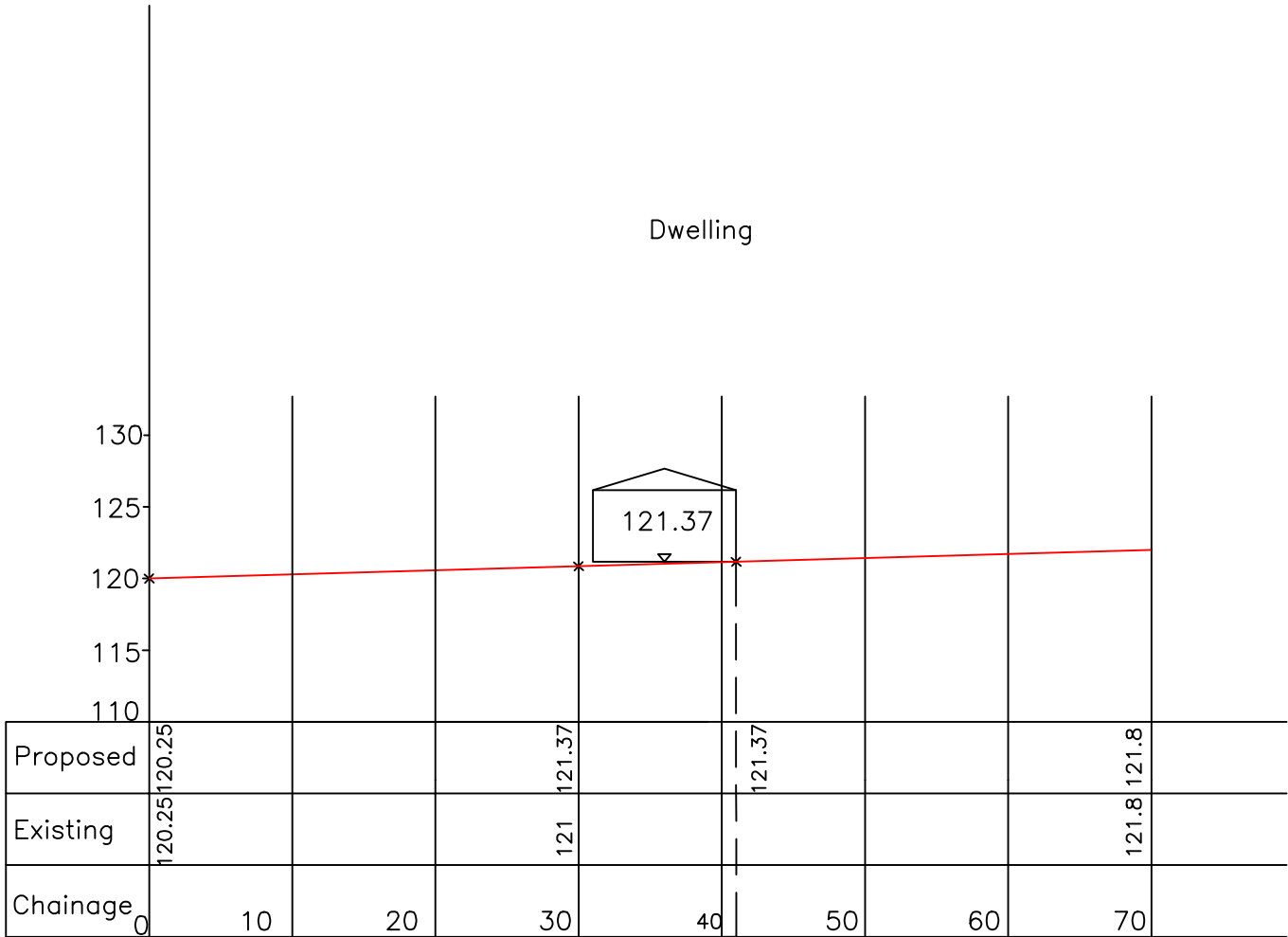
Section Y–Y
