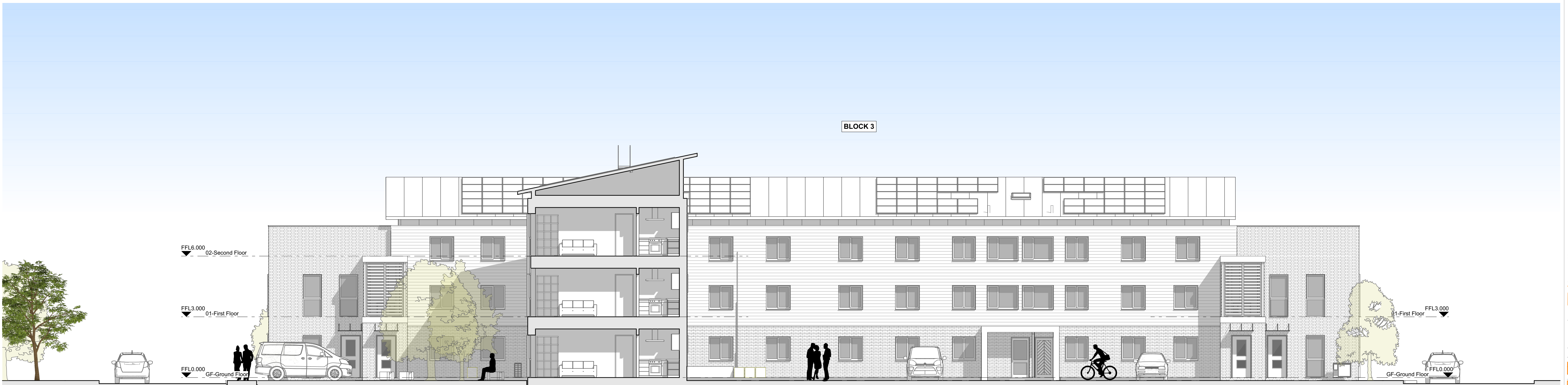
S-04 Block 3 Courtyard Section
