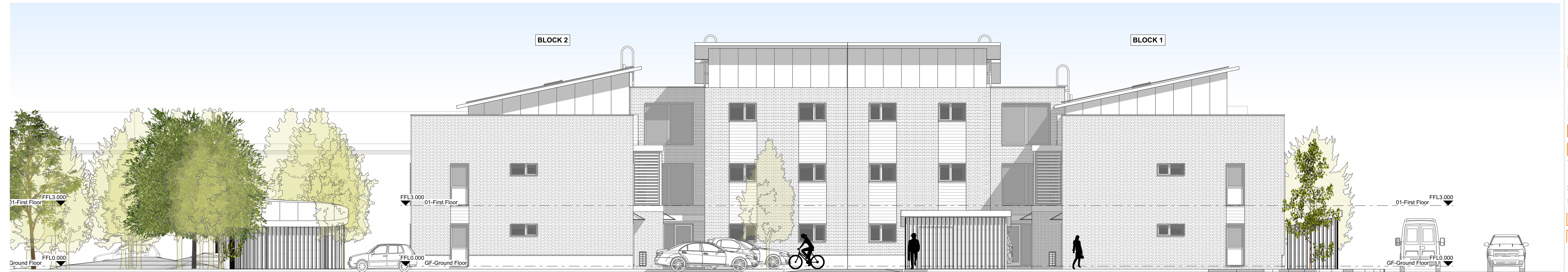
E-03 Moorland Road Elevation
