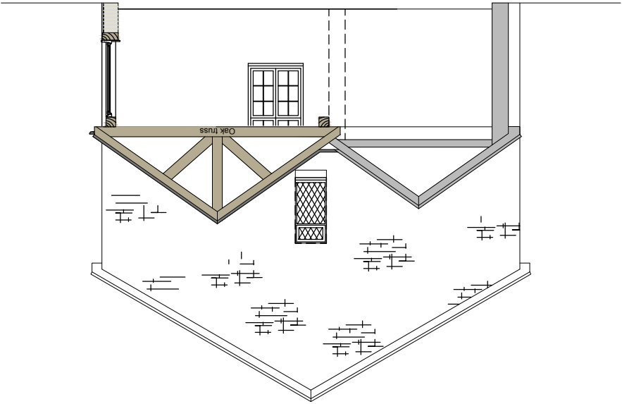
PROPOSED SECTION
