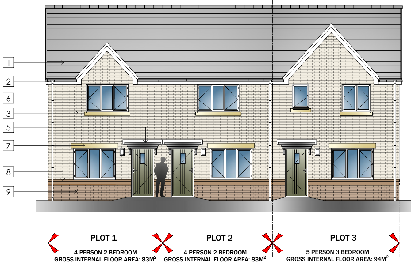
FRONT ELEVATION
