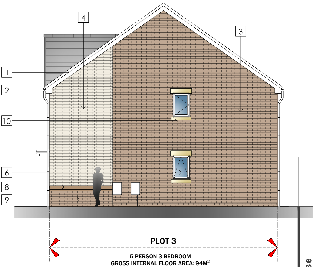
SIDE ELEVATION
