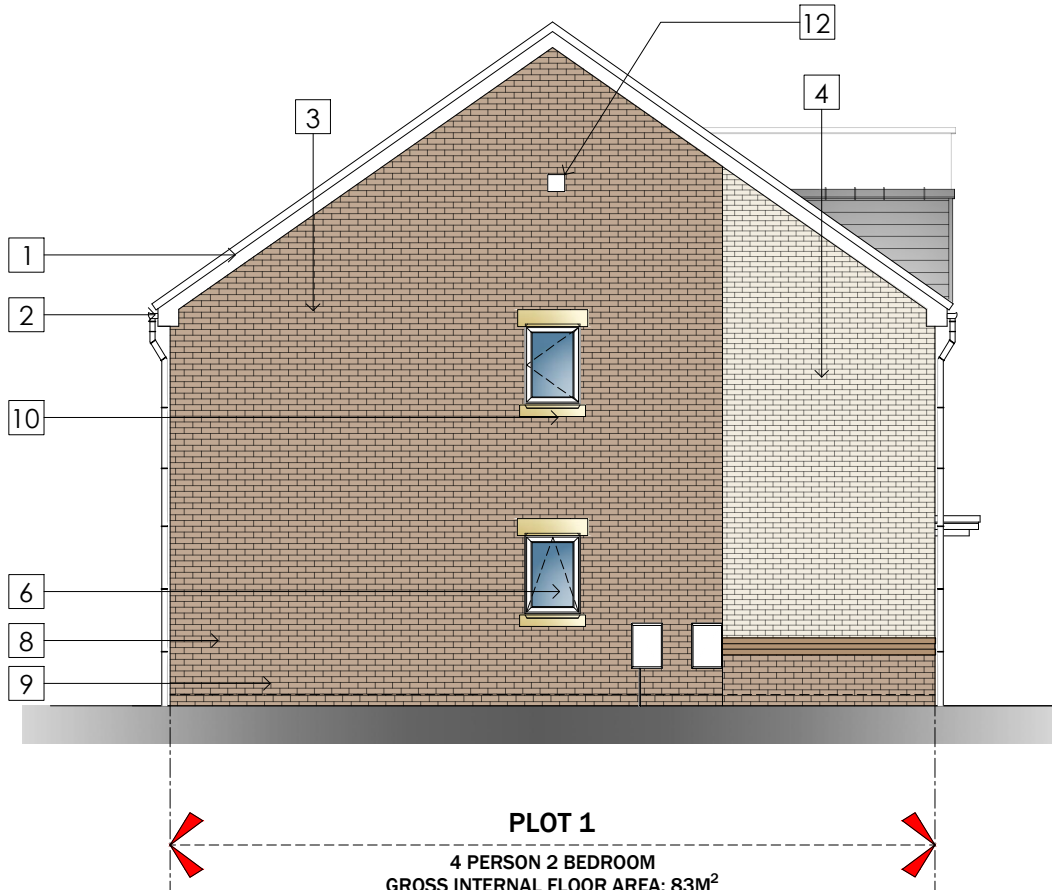
SIDE ELEVATION
