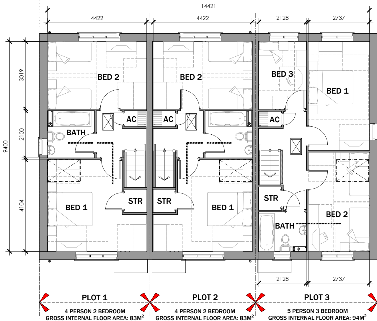
GROUND FLOOR
