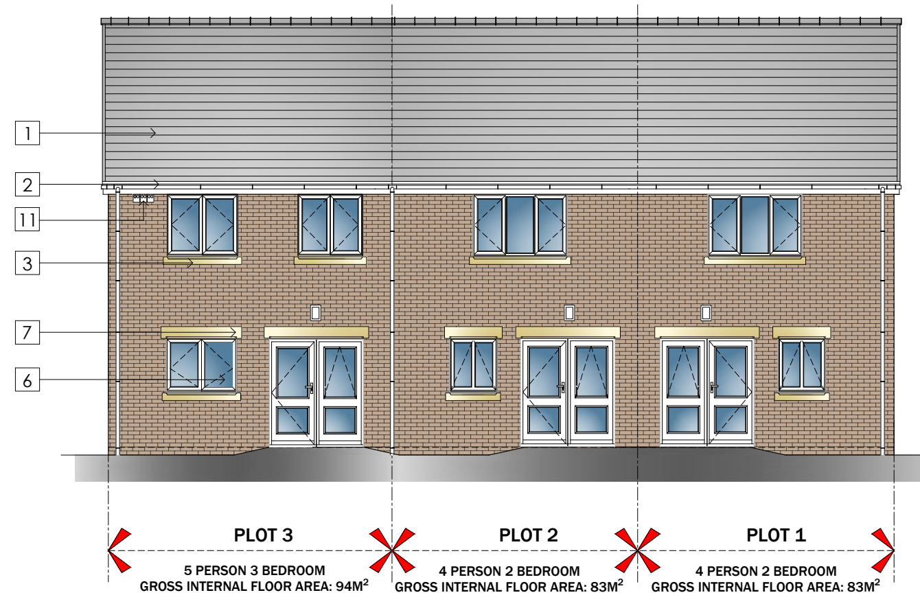
REAR ELEVATION
