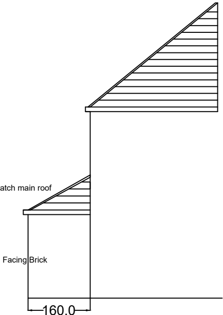
Proposed LHS Elevation
