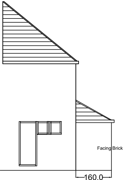
Proposed RHS Elevation
