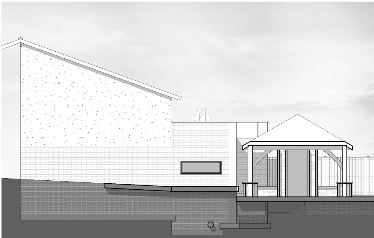
Proposed RHS Elevation 1 : 100
