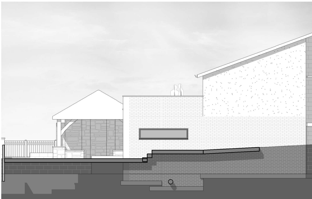
Proposed LHS Elevation 1 : 100
