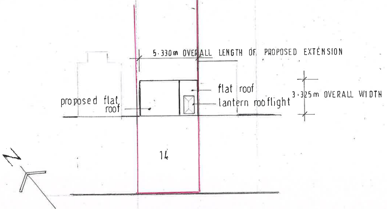
PROPOSED ROOF PLAN scale 1 : 200
