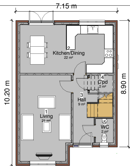
1 Plot 1 - GF 1 : 100
