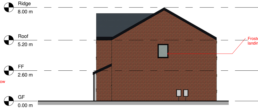
2 Plot 1 - East 1 : 100
