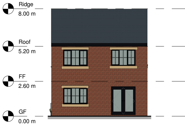
3 Plot 1 - South 1 : 100
