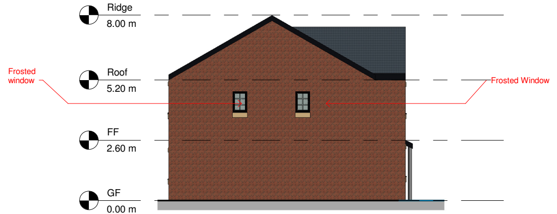
4 Plot 1 - West 1 : 100
