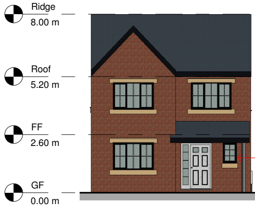
1 Plot 1 - North 1 : 100
