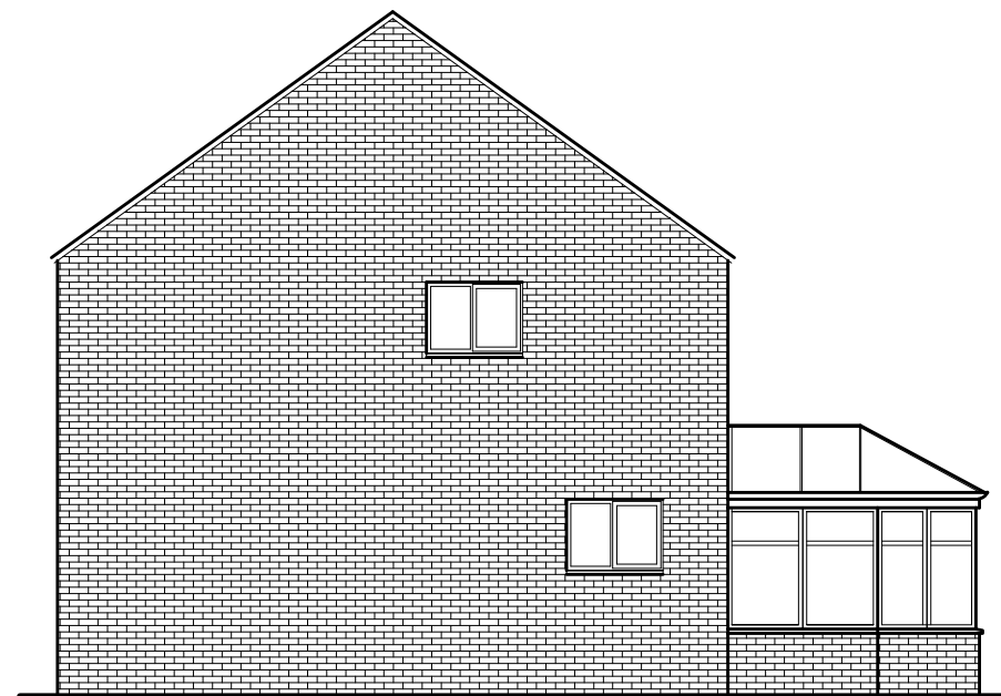
Existing RH Side Elevation
