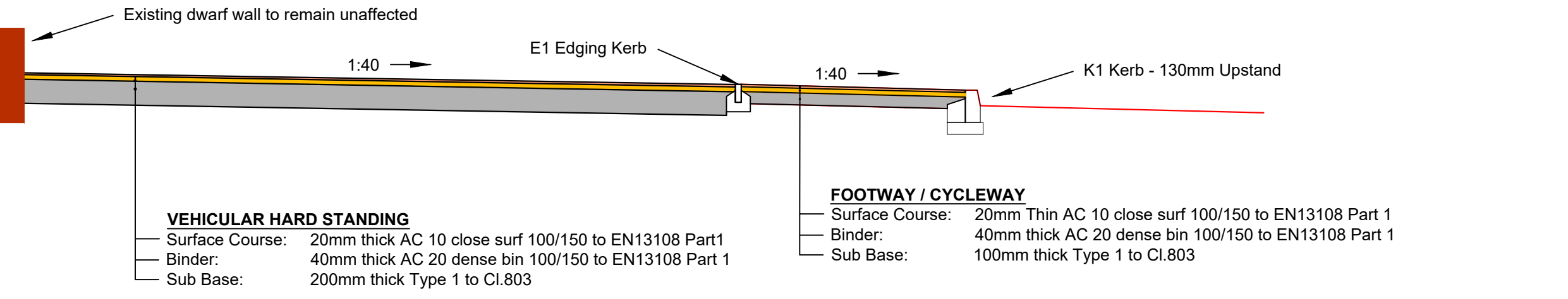
TYPICAL SECTION C-C
