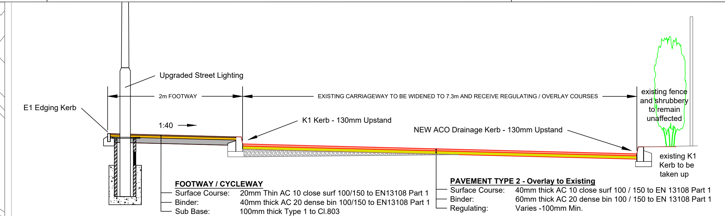
TYPICAL SECTION B-B
