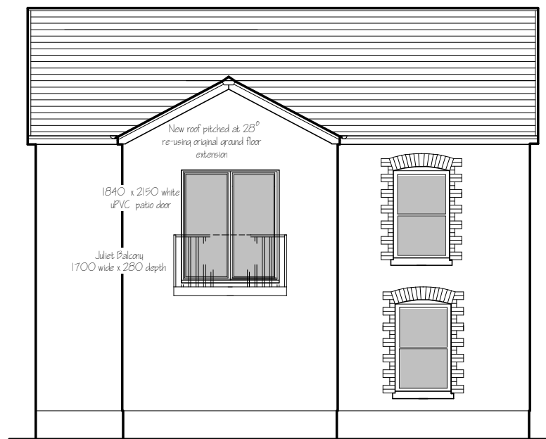
REAR ELEVATION Facing North
