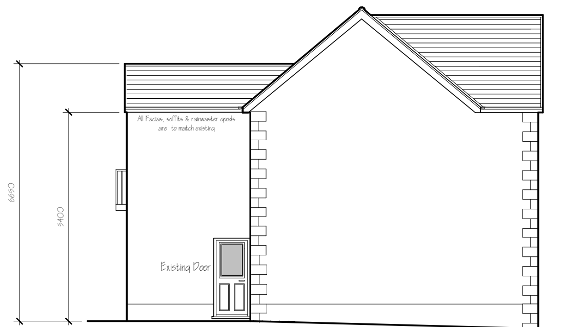
SIDE ELEVATION Facing West
