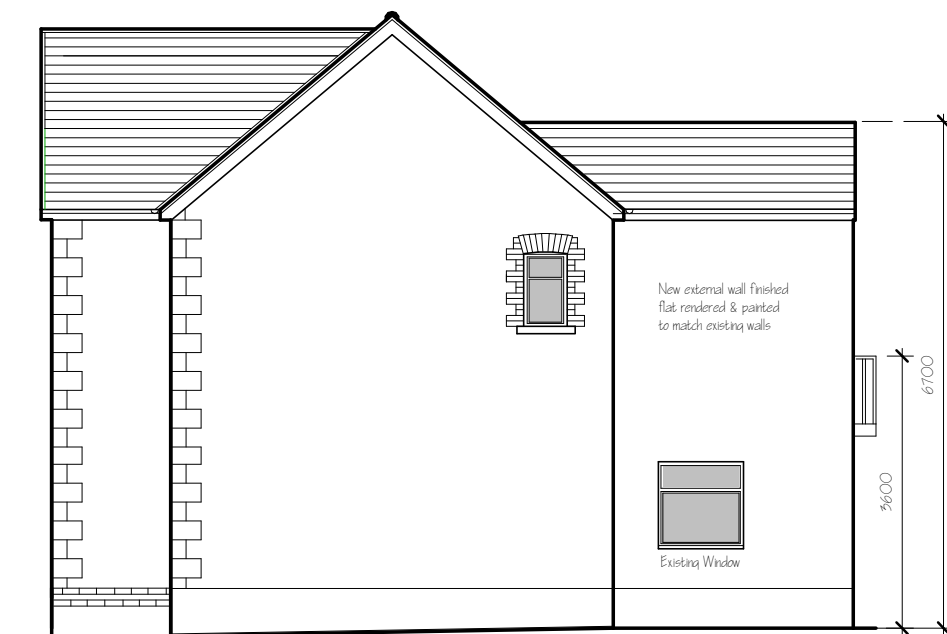
SIDE ELEVATION Facing East
