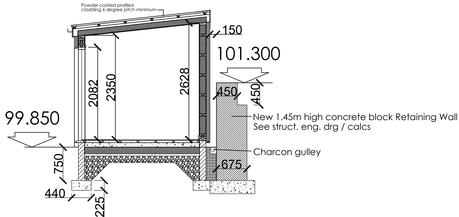
PROPOSED SECTION 1:50 SCALE B-04a 1A WELLS CLOSE
