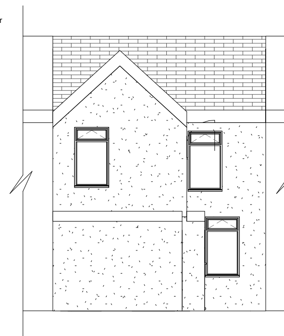
Existing South 1 : 100
