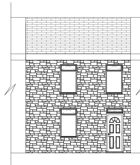
Existing North 1 : 100
