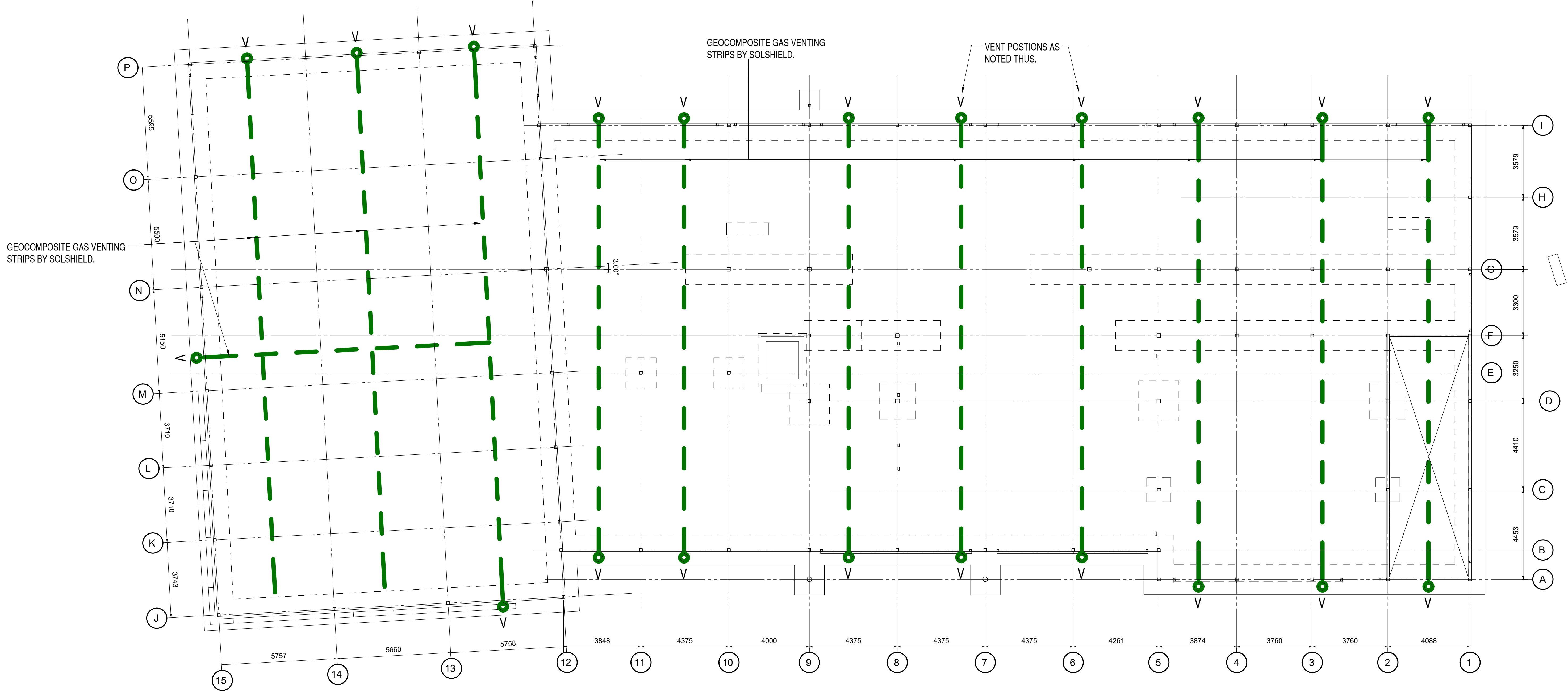
PLAN GROUND FLOOR GAS VENTING. ( 1 : 100 )
