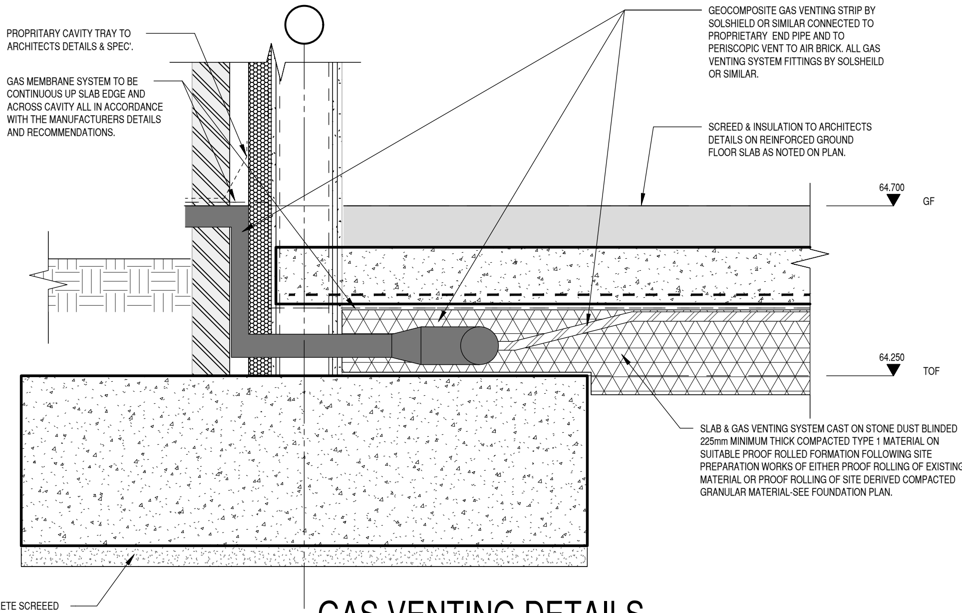
GAS VENTING DETAILS. ( 1 : 10 )
