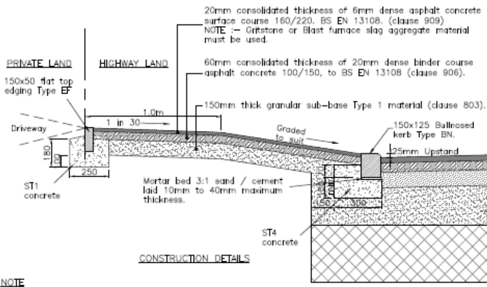
ELEVATION OF VEHICULAR CROSSOVER
