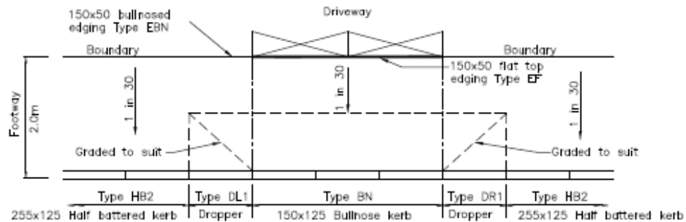
PLAN OF VEHICULAR CROSSOVER
