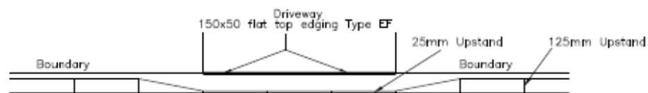
ELEVATION OF VEHICULAR CROSSOVER
